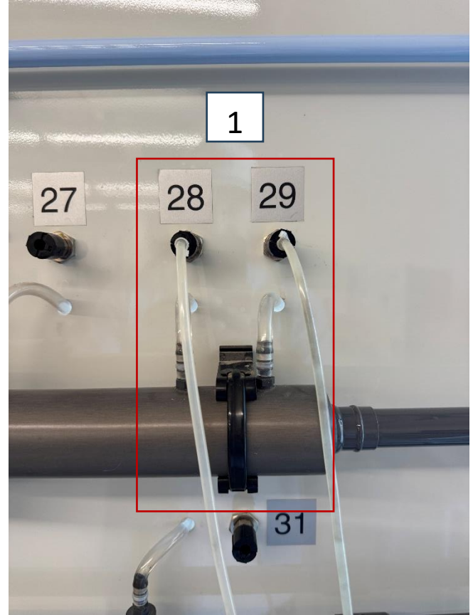
Figure 2 Shows the Venturi tapping that was used (1).
