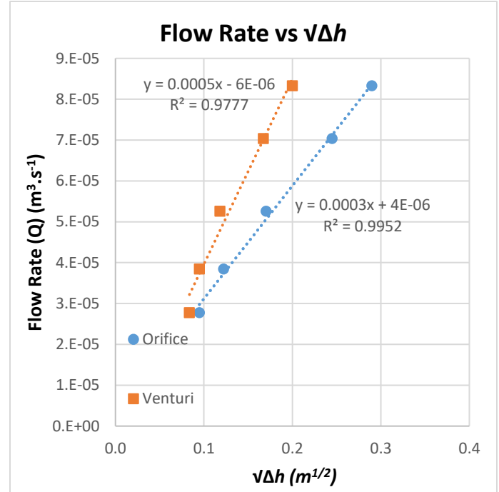
Figure 4 Flow rate ( Q ) vs. \sqrt{\Delta h} for Venturi and Orifice meters.
