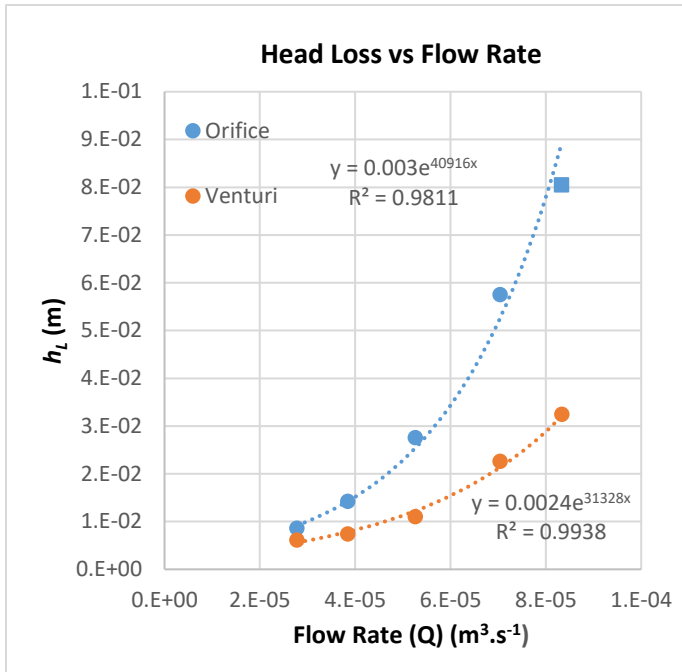
Figure 7 Head loss vs flow rate comparison.
