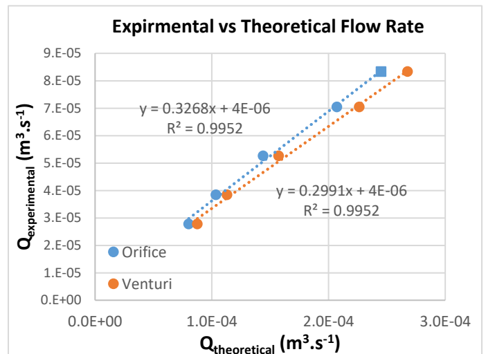
Figure 6 Experimental vs theoretical flow rate comparison.
