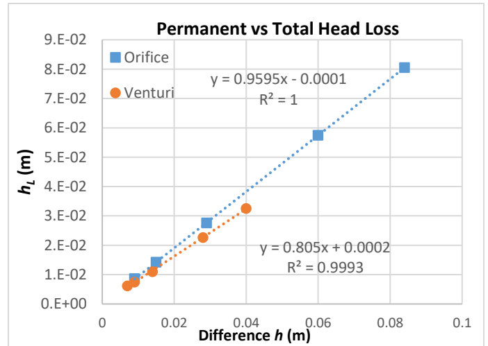
Figure 5 Permanent head loss ( h_L ) versus total pressure drop ( \Delta h ).
